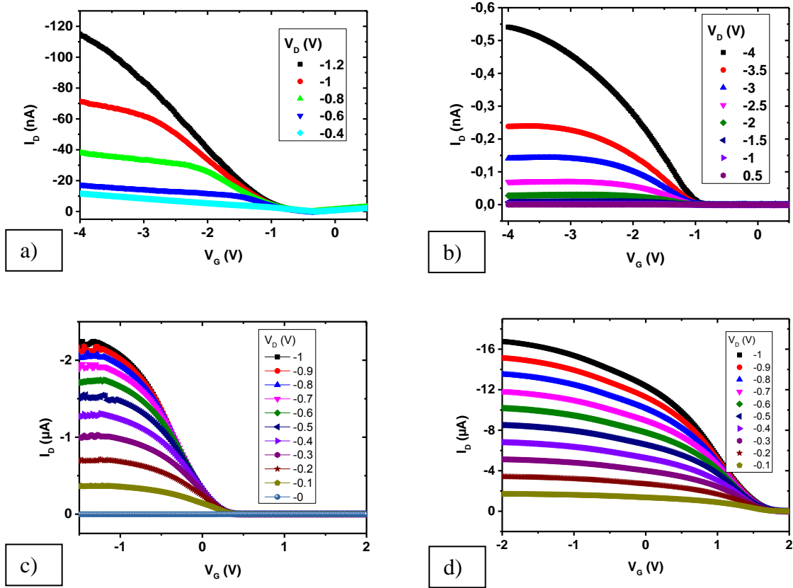
Fig. 6 Drain current ( I_D ) vs. gate voltage ( V_G ) for pMOSFETs prepared in p-type silicon (a,b) and n-type silicon (c,d). Figs. (a) and (c) are from measurements on reference devices without dislocations, while Figs. (b) and (d) are obtained from devices with dislocations in the channel. Note the different scale.
