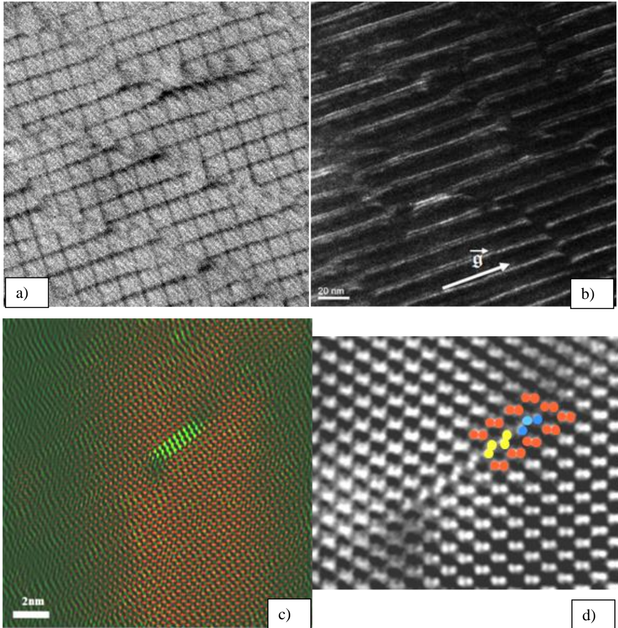
Fig. 2 Scanning transmission electron microscope (STEM) plan-view image of a screw dislocation network formed by wafer bonding of Si(100) wafers (a). Weak beam image of one set of dislocations (b). HAADF-STEM image of a dissociated screw dislocation (c). The image was color coded for clearness. A part of the defect is shown at higher magnification in (d). Red dots characterize dumbbells of the (undisturbed) Si matrix, while blue and yellow dots characterize dumbbells at the partial dislocation and stacking fault, respectively. Samples with \langle 100 \rangle orientation were used for Figures (a) and (b), while Figures (c) and (d) were produced from \langle 110 \rangle oriented cross sections of the same dislocation network.
