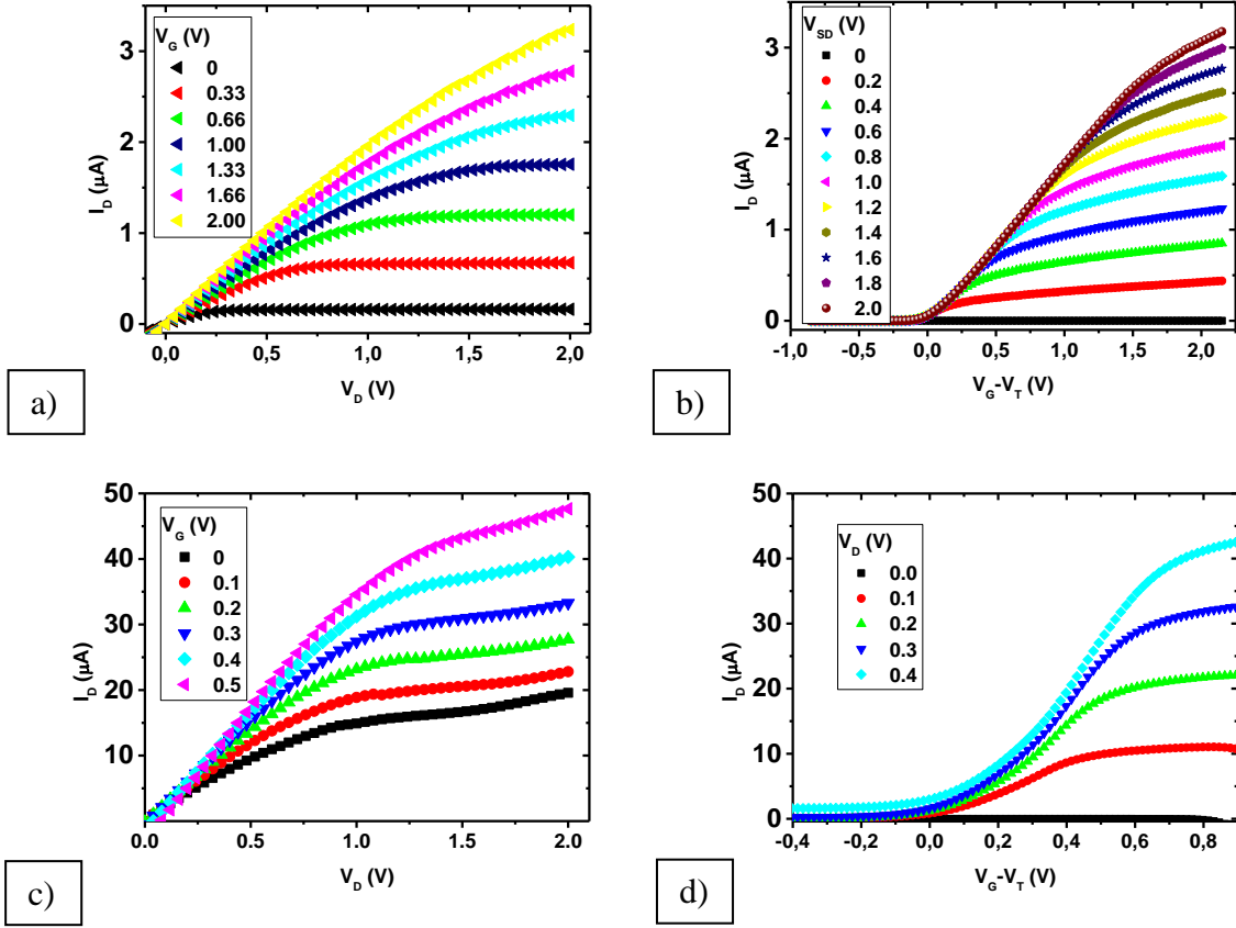
Fig. 5 Output and transfer characteristics of nMOSFETs without dislocations (a,b) and with a dislocation network (c,d). The device layer thickness was 80 nm. The channel length and width, respectively, for both devices are 1 \mu\text{m} . Caused by the different threshold voltages ( V_T ) of both devices, the gate voltage ( V_G ) is represented for clarity as V_G - V_T .
