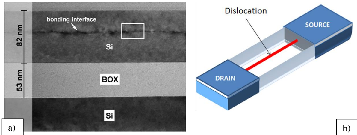
Fig. 4 TEM cross-section image of a SOI substrate with a dislocation network in the device layer (a). The dislocation distance is about 15 nm corresponding to a twist angle of about 0.7^\circ . Scheme of a MOSFET having a dislocation in the channel (b). Because dislocations are parallel to \langle 110 \rangle -directions in Si, they are parallel to the channel and source and drain form electrical contacts. The gate electrode is not shown in the scheme.
